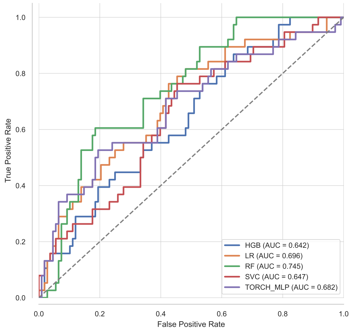
Combined ROC Curve (New neurological deficits)
